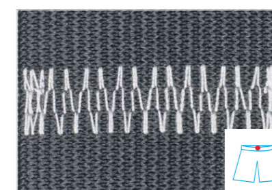
Elastic joint P31
