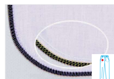
Five threads pocket double chain rolling stitch P15
