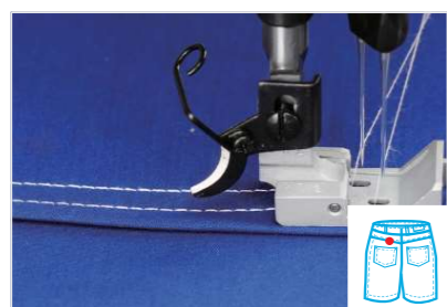
Double needle chain stitch P10
