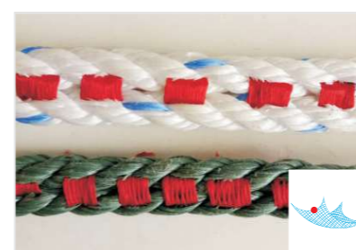
Fishing net P31
